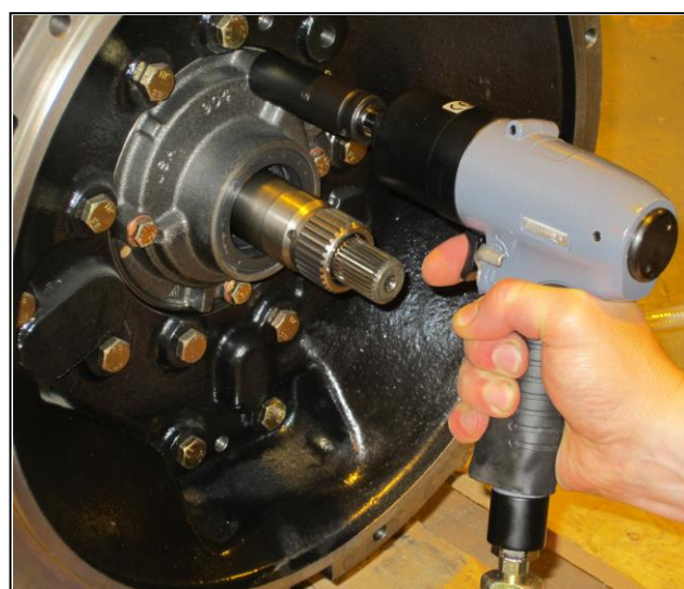
Example application – assembly of gearbox on mass production line
